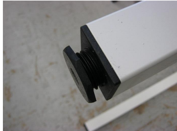
Photo 6: Tested sample 220609-2 of Techo Fount Classic N-Leg office desk - detail final leveller
